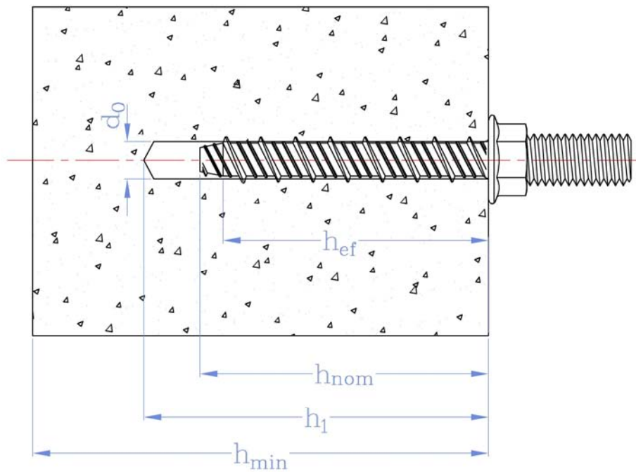
Drawing A3. Installed condition for anchors SSD, SSI, SSF, SSO, SSU, SSG, SSQ and SSV
