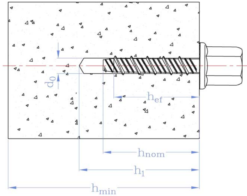
Drawing A2. Installed condition for anchors SSD, SSI, SSF, SSO, SSU, SSG, SSQ and SSV
